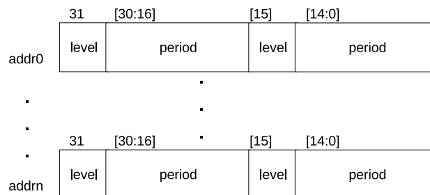
Figure 30.2-2. Data Structure
