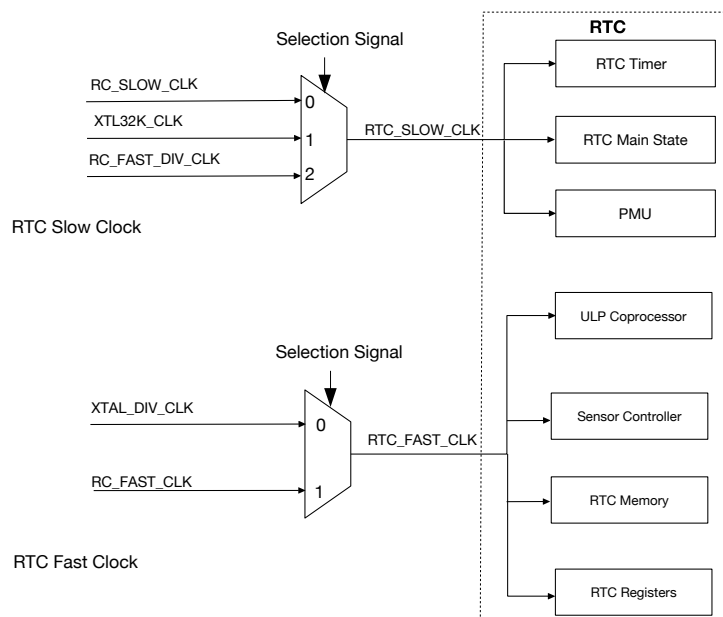
Figure 9.3-6. RTC Low-Power Clocks
