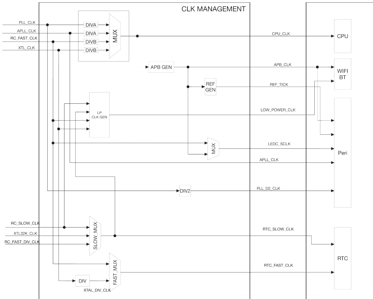
Figure 7.2-1. System Clock
