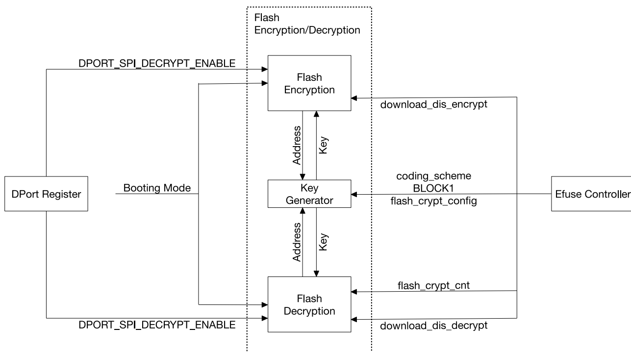
Figure 17.3-1. Flash Encryption/Decryption Module Architecture
