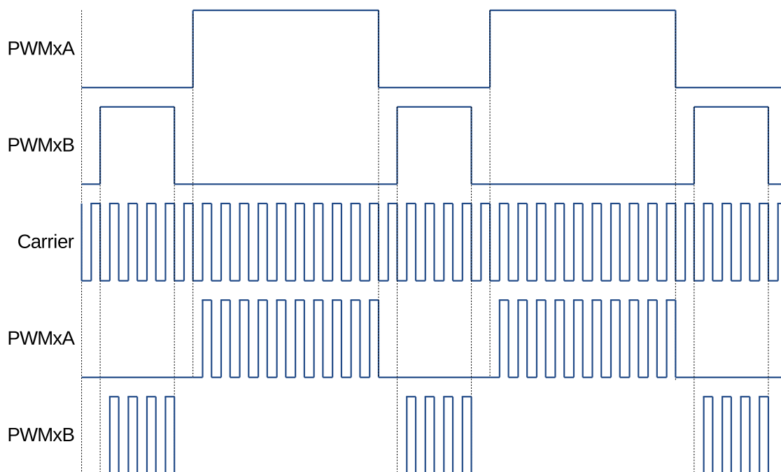
Figure 29.3-26. Example of Waveforms Showing PWM Carrier Action
