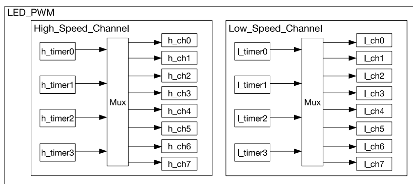
Figure 28.2-1. LED_PWM Architecture
