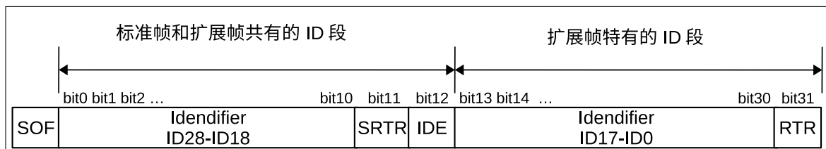
Figure 25.5-5. Positions of Arbitration Lost Bits
