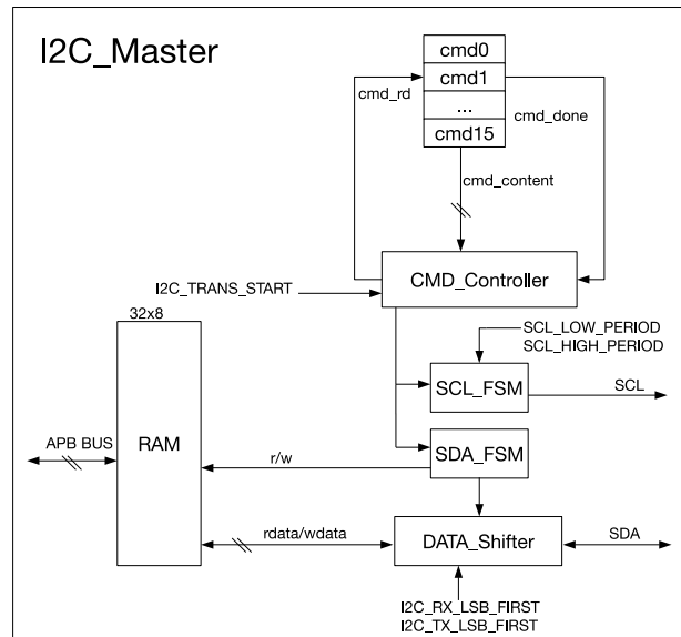
Figure 21.3-1. I2C Master Architecture
