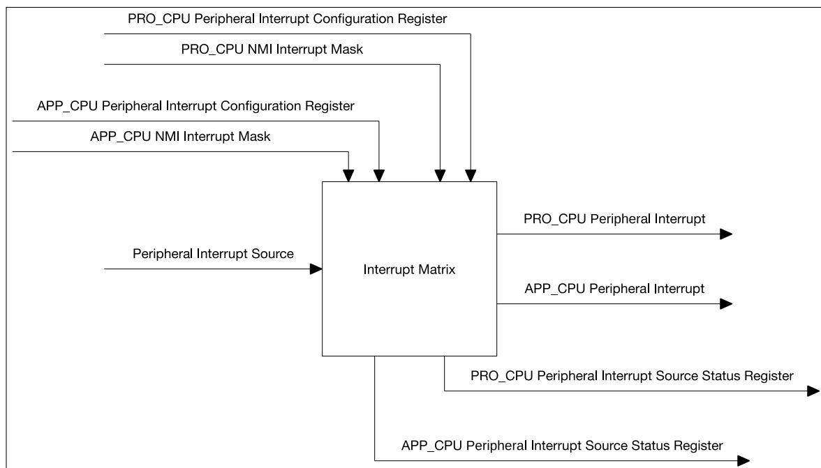
Figure 8.2-1. Interrupt Matrix Structure
