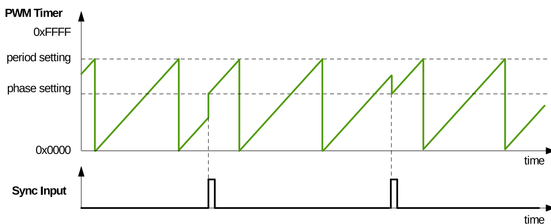
Figure 29.3-6. Count-Up Mode Waveform
