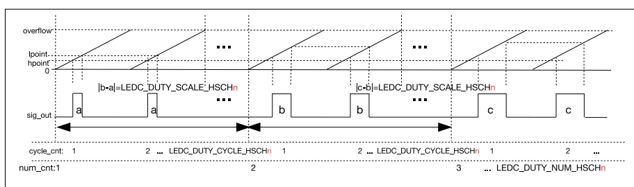
Figure 28.2-5. Output Signal Diagram of Fading Duty Cycle
