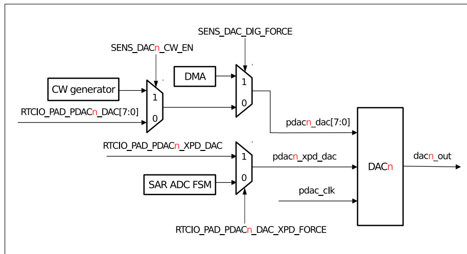
Figure 31.4-1. Diagram of DAC Function
