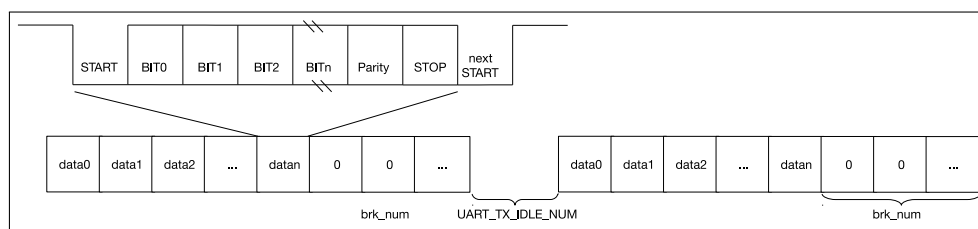
Figure 19.3-3. UART Data Frame Structure
