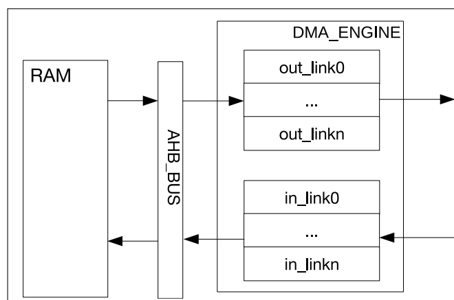
Figure 2.3-1. DMA Engine Architecture
