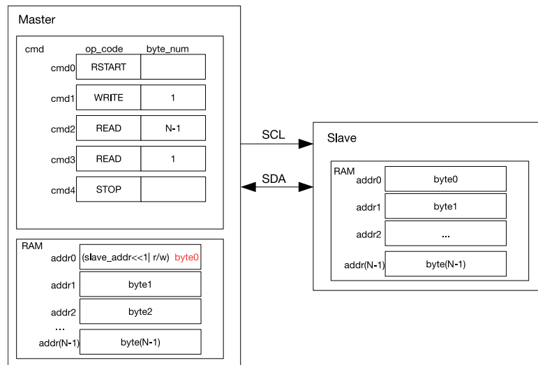
Figure 21.3-9. Master Reads from Slave with 7-bit Address
