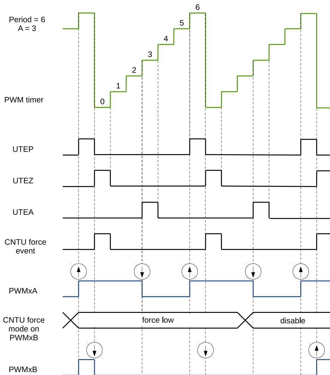
Figure 29.3-20. Example of a CNTU Software-Force Event on PWMxB
