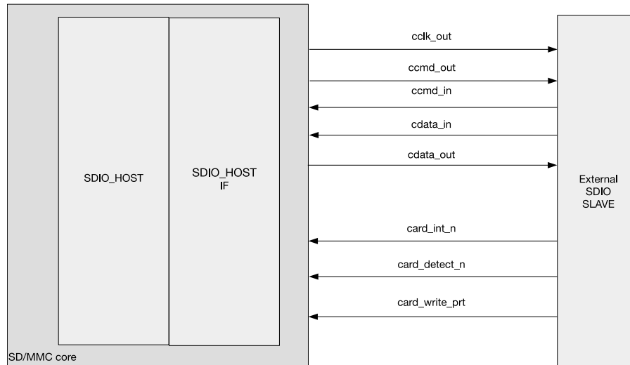
Figure 27.3-1. SD/MMC Controller External Interface Signals
