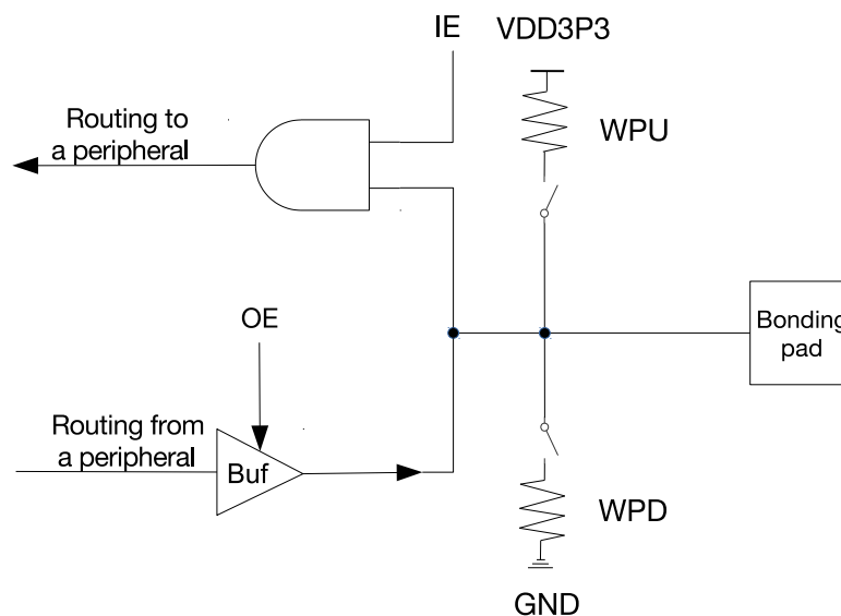
Figure 6.1-2. Internal Structure of a Pad
