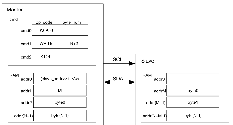
Figure 21.3-7. I2C Master Writes to addrM in RAM of Slave with 7-bit Address
