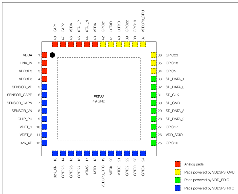
Figure 6.8-1. ESP32 I/O Pin Power Sources (QFN 6*6, Top View)
