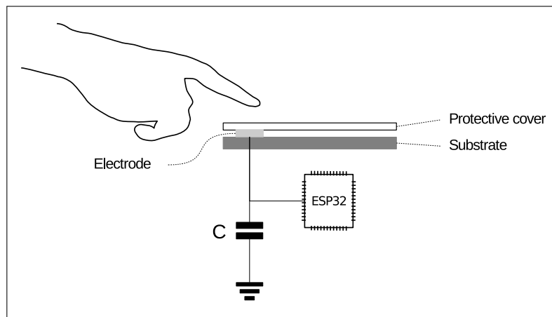
Figure 31.2-1. Touch Sensor
