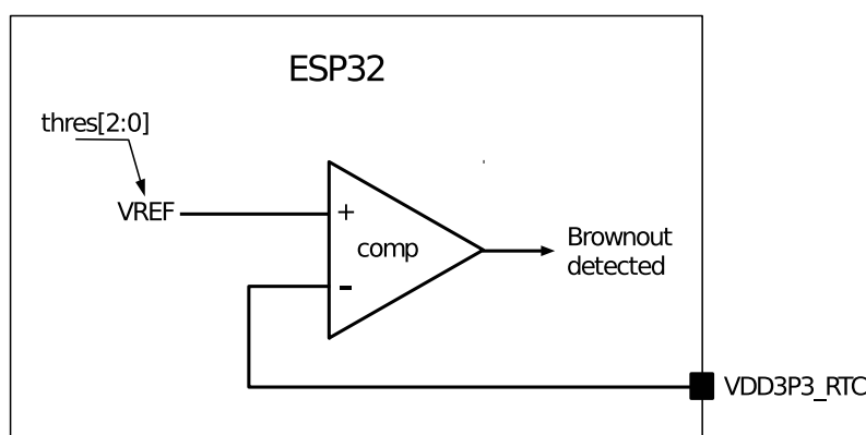
Figure 9.3-4. Brownout Detector
