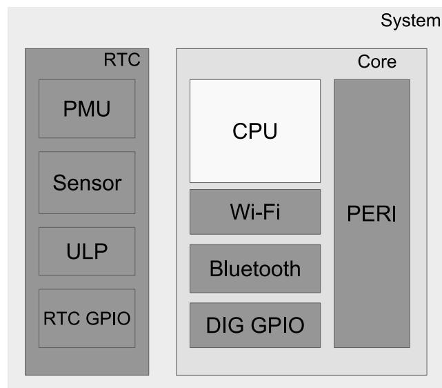
Figure 7.1-1. System Reset
