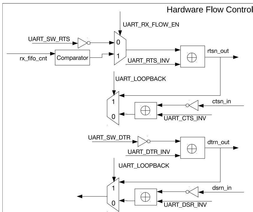
Figure 19.3-5. Hardware Flow Control
