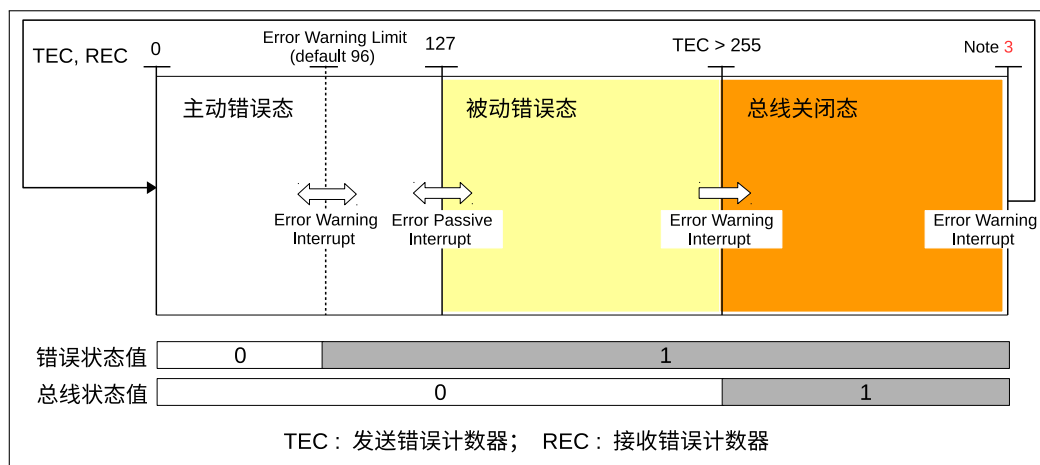
Figure 25.5-4. Error State Transition
