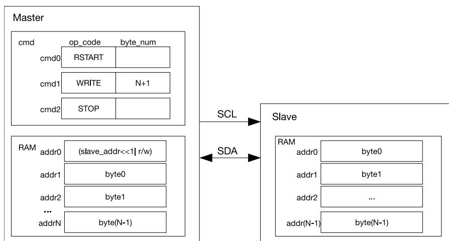
Figure 21.3-5. I2C Master Writes to Slave with 7-bit Address
