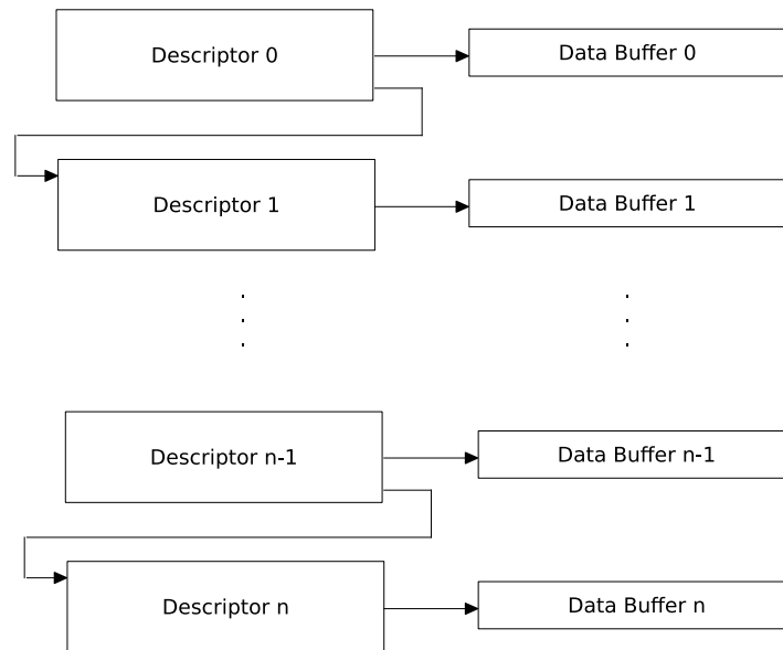
Figure 26.3-5. SDIO Slave Linked List
