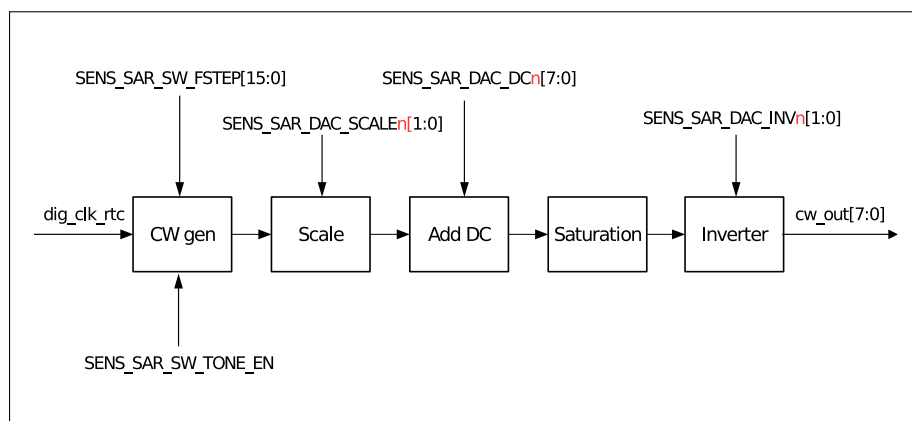
Figure 31.4-2. Cosine Waveform (CW) Generator
