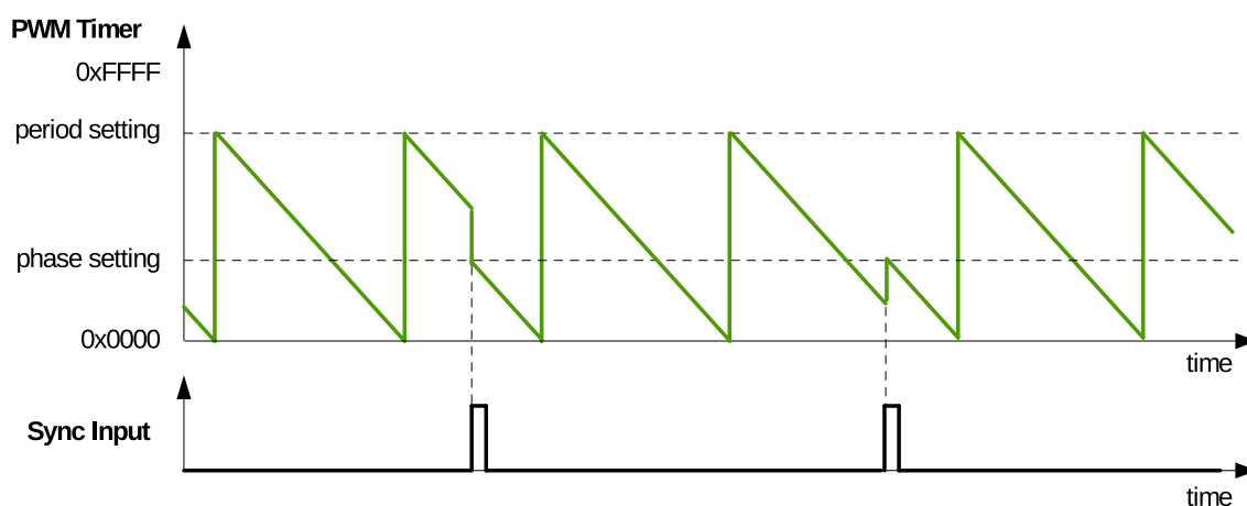
Figure 29.3-7. Count-Down Mode Waveforms
