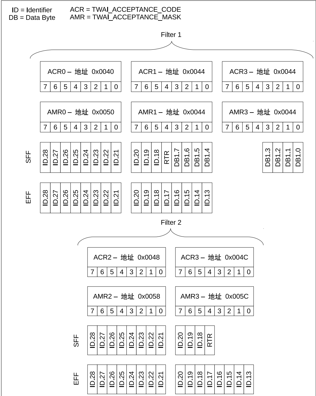
Figure 25.5-3. Dual Filter Mode
