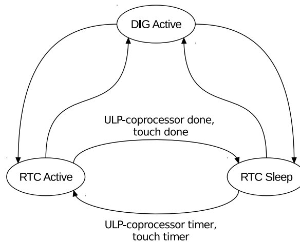
Figure 9.3-8. RTC States
