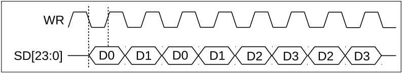
Figure 22.5-3. LCD Master Transmitting Data Frame, Form 2
