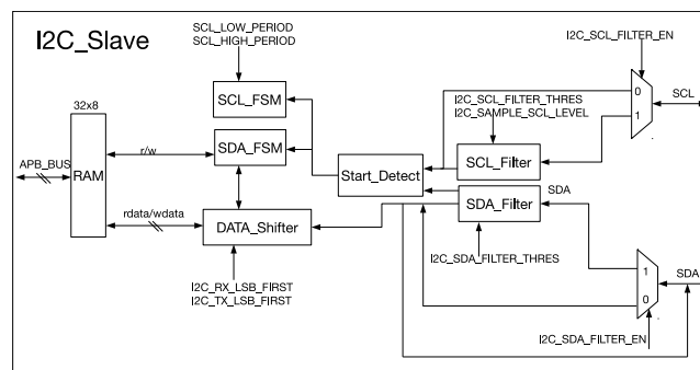
Figure 21.3-2. I2C Slave Architecture
