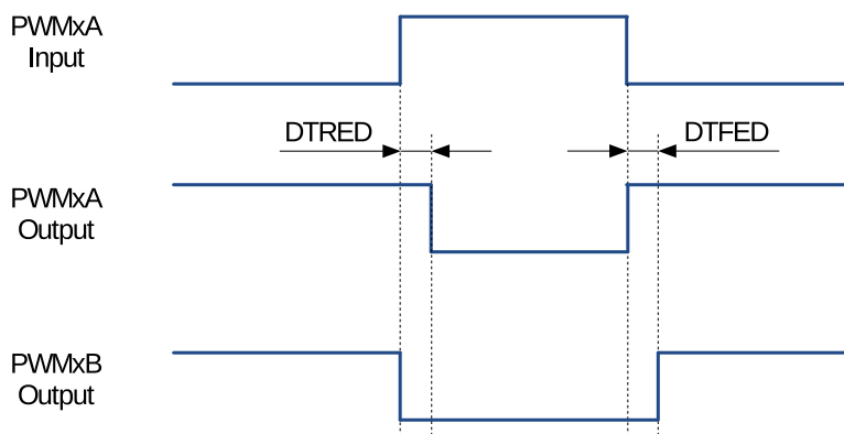
Figure 29.3-25. Active Low (AL) Dead Time Waveforms
