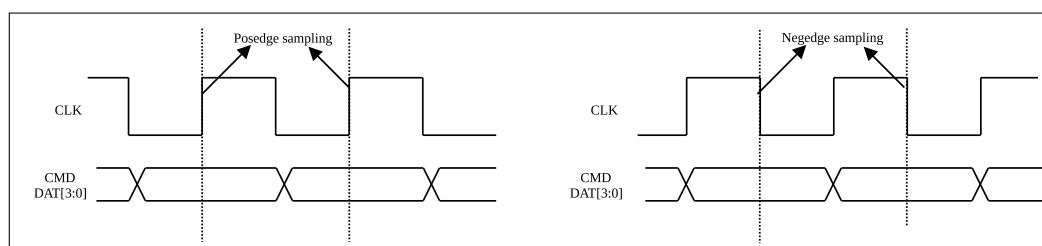
Figure 26.3-9. Sampling Timing Diagram
