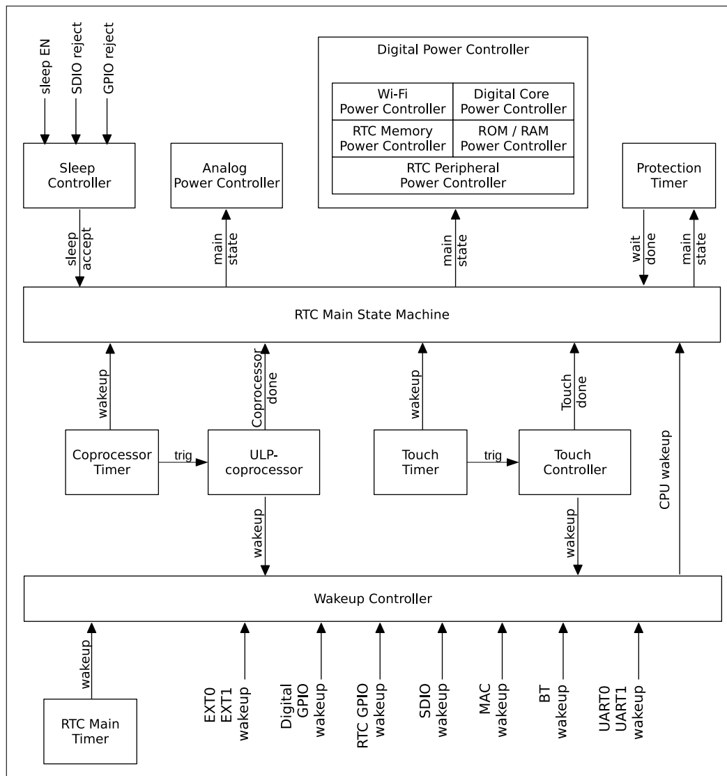
Figure 9.3-5. RTC Structure
