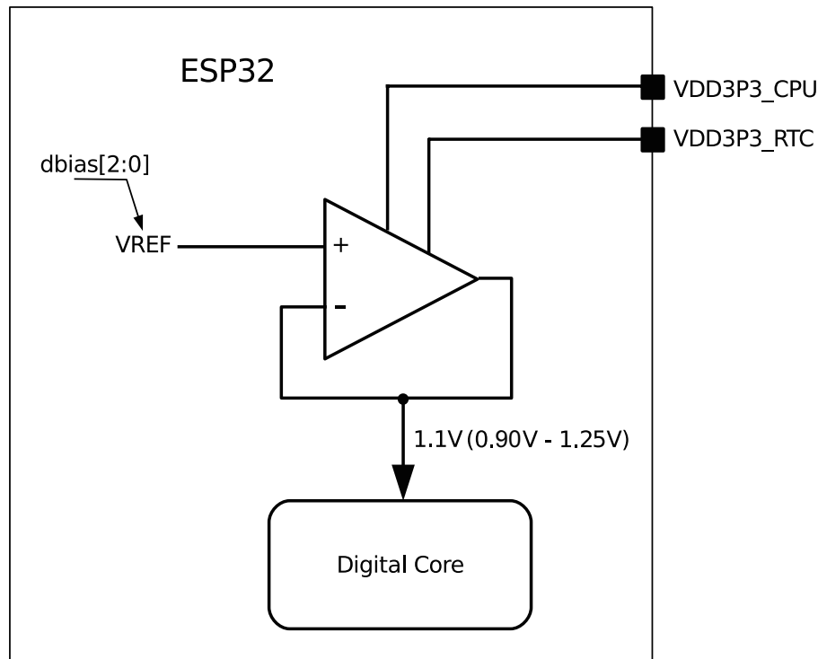
Figure 9.3-1. Digital Core Voltage Regulator
