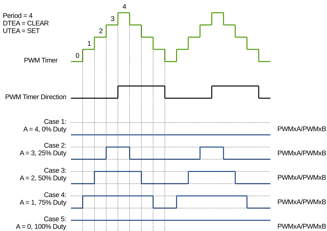
Figure 29.3-14. Symmetrical Waveform in Count-Up-Down Mode
