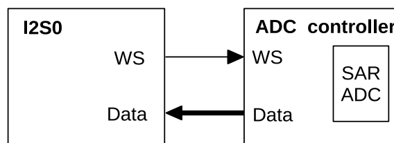
Figure 22.5-5. ADC Interface of I2S0
