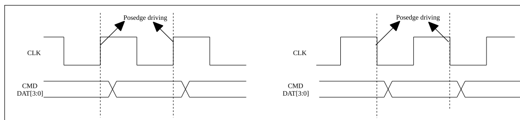
Figure 26.3-10. Output Timing Diagram
