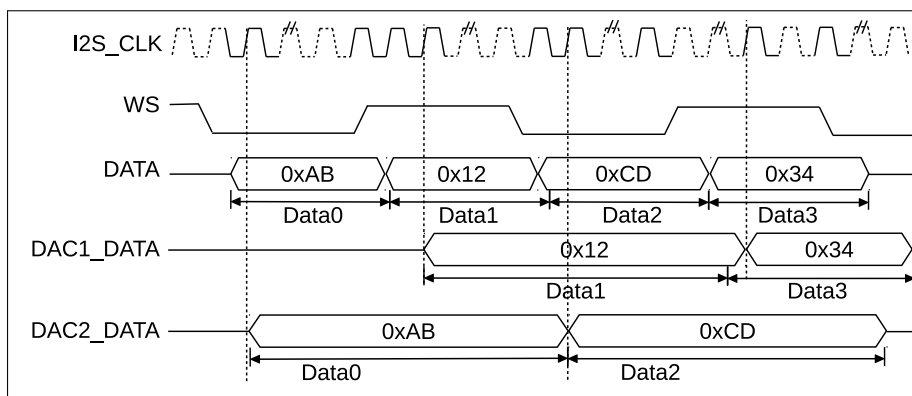
Figure 22.5-7. Data Input by I2S DAC Interface
