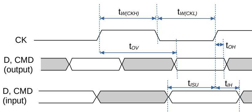
Figure 27.10-1. SD/MMC Timing in HS Mode
