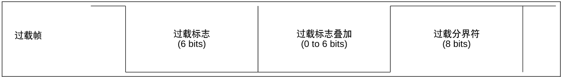
Figure 25.3-3. The Bit Fields of an Overload Frame
