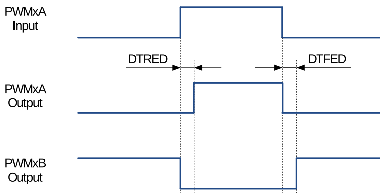
Figure 29.3-22. Active High Complementary (AHC) Dead Time Waveforms
