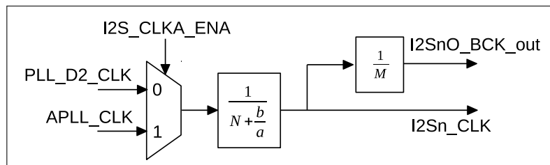
Figure 22.3-1. I2S Clock
