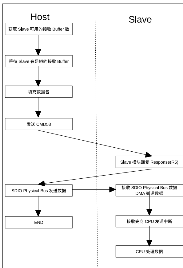
Figure 26.3-7. Packet Receiving Procedure (Initiated by Host)
