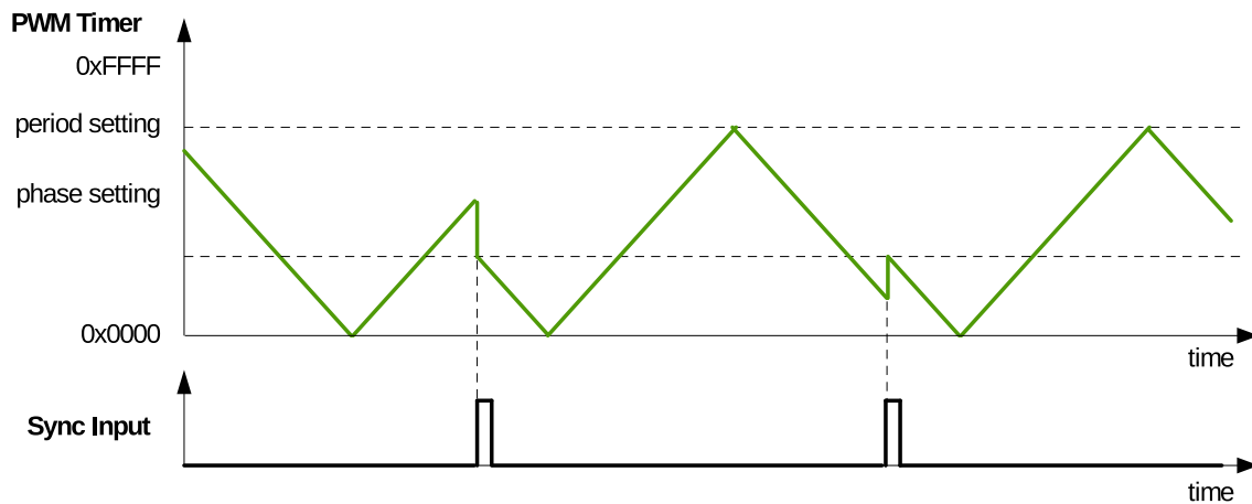
Figure 29.3-8. Count-Up-Down Mode Waveforms, Count-Down at Synchronization Event
