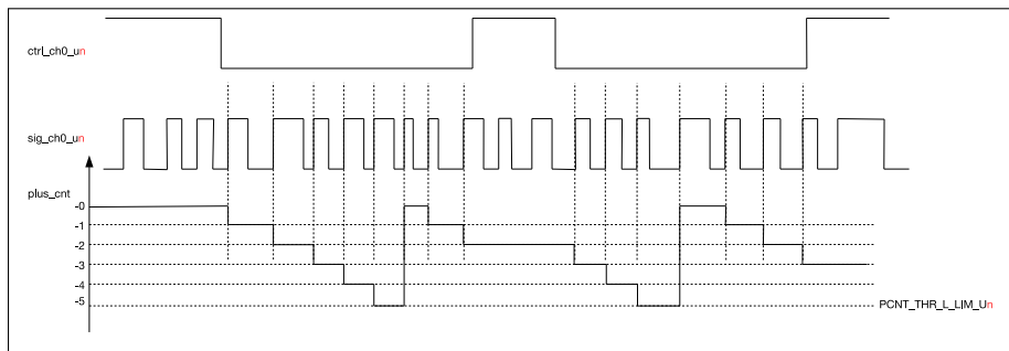
Figure 23.2-3. PULSE_CNT Downcounting Diagram
