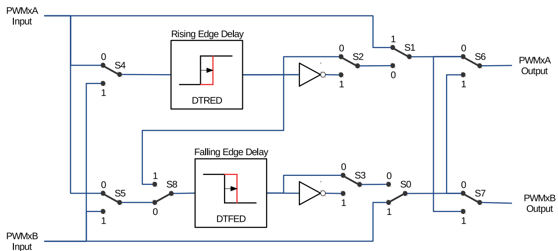
Figure 29.3-21. Options for Setting up the Dead Time Generator Submodule
