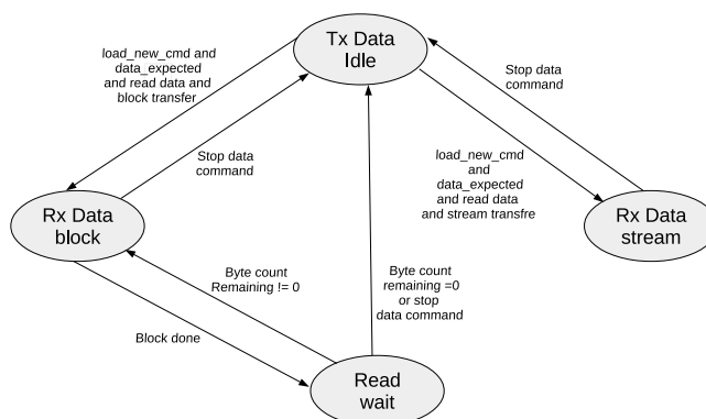
Figure 27.4-4. Data Receive State Machine
