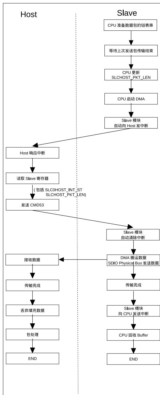
Figure 26.3-6. Packet Sending Procedure (Initiated by Slave)
