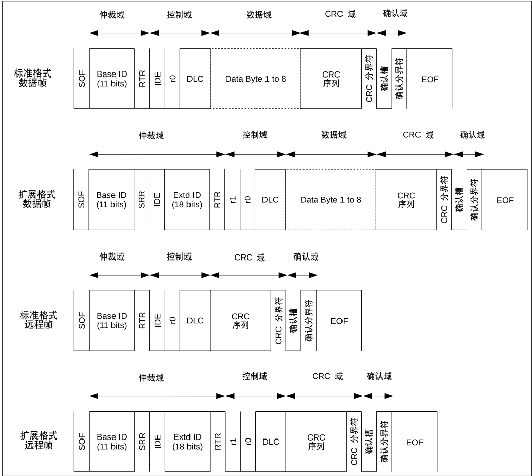
Figure 25.3-1. The bit fields of Data Frames and Remote Frames
