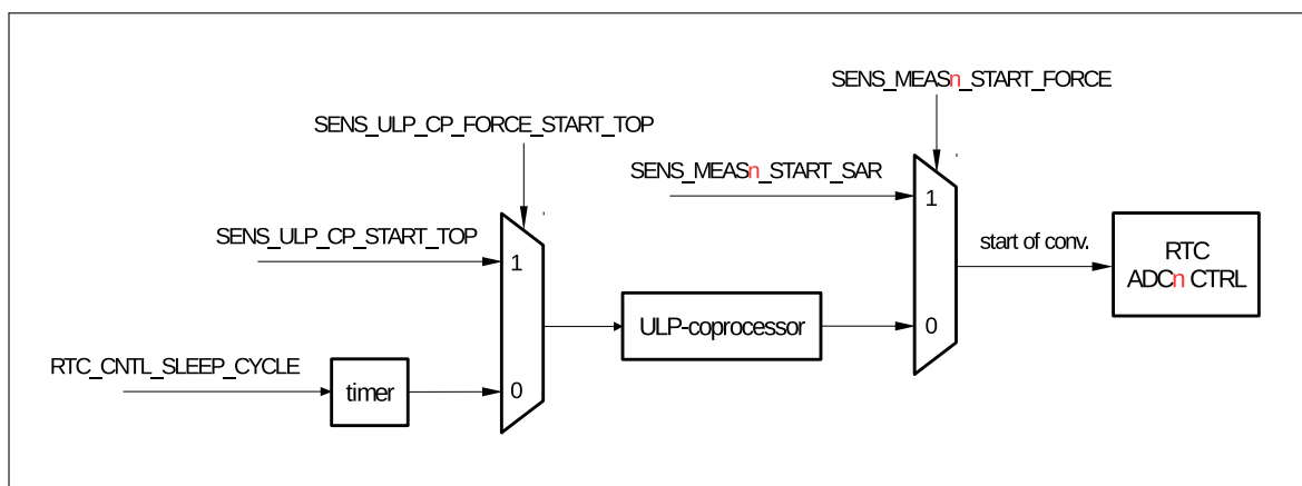
Figure 31.3-3. RTC SAR ADC Outline of Function
