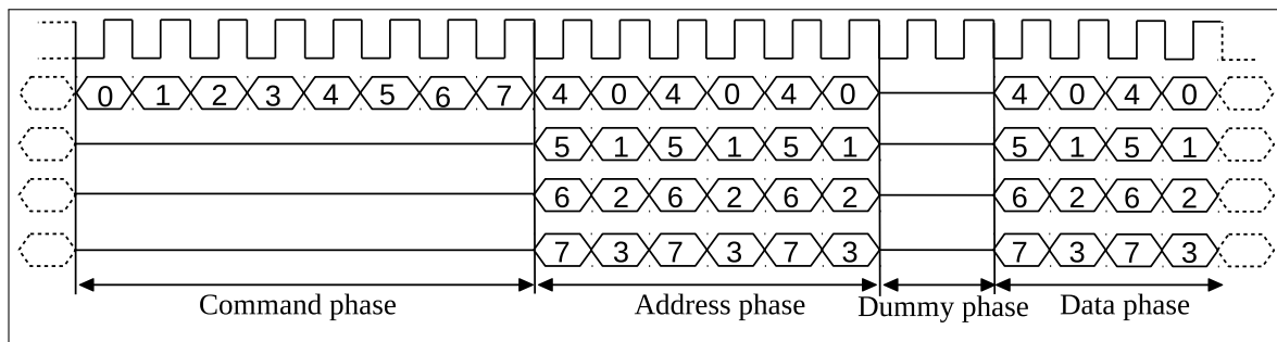
Figure 20.5-2. Communication Format of Parallel QSPI
