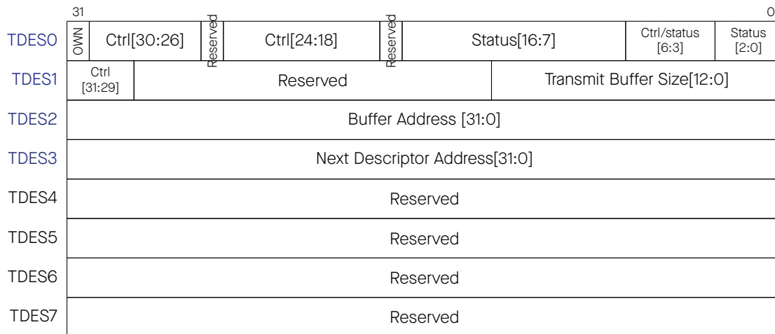
Figure 24.8-1. Transmit Descriptor
