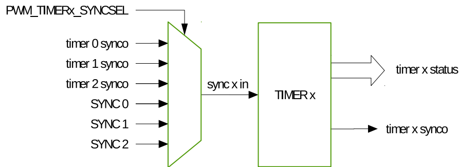
Figure 29.3-2. Timer Submodule
