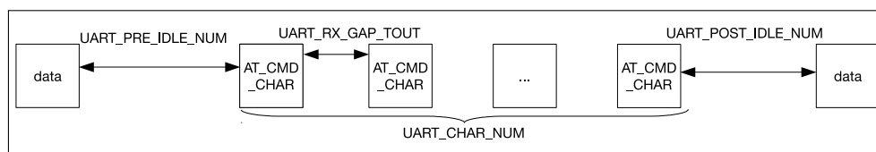
Figure 19.3-4. AT_CMD Character Format
