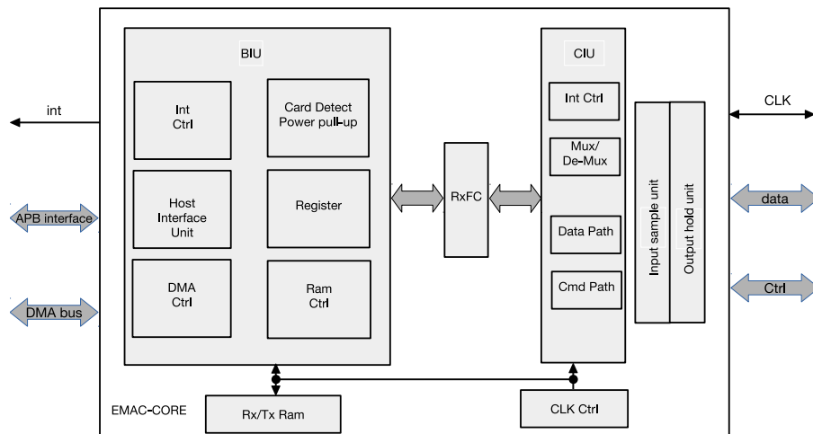
Figure 27.4-1. SDIO Host Block Diagram
