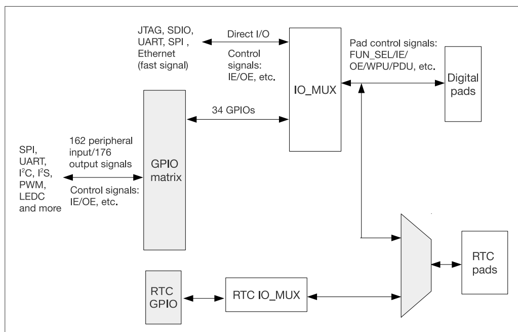
Figure 6.1-1. IO MUX, RTC IO MUX and GPIO Matrix Overview
