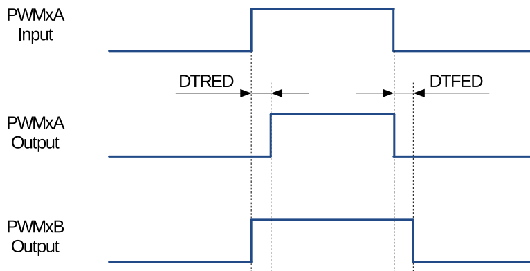
Figure 29.3-24. Active High (AH) Dead Time Waveforms
