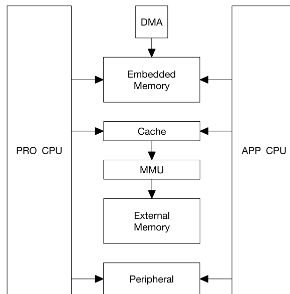
Figure 3.2-1. System Structure
