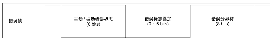
Figure 25.3-2. Various Fields of an Error Frame
