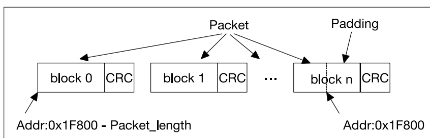
Figure 26.3-2. SDIO Bus Packet Transmission
