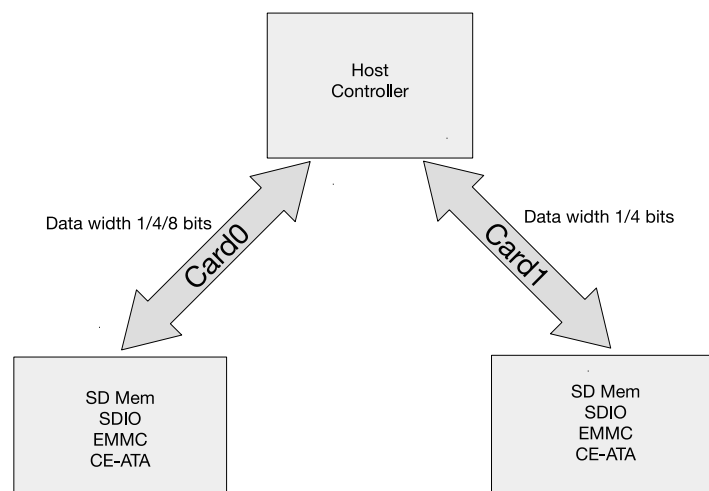
Figure 27.2-1. SD/MMC Controller Topology
