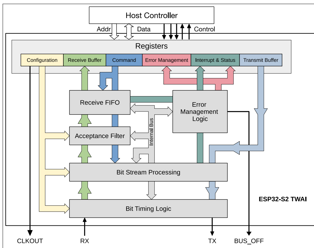
Figure 25.4-1. TWAI Overview Diagram
