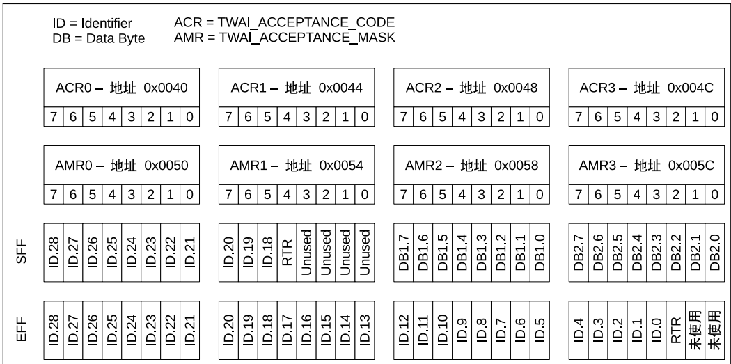
Figure 25.5-2. Single Filter Mode
