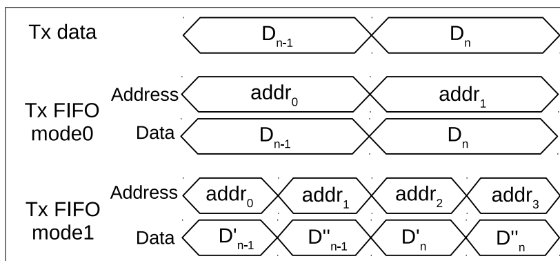
Figure 22.4-4. Tx FIFO Data Mode
