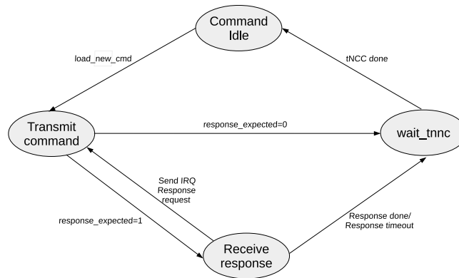
Figure 27.4-2. Command Path State Machine
