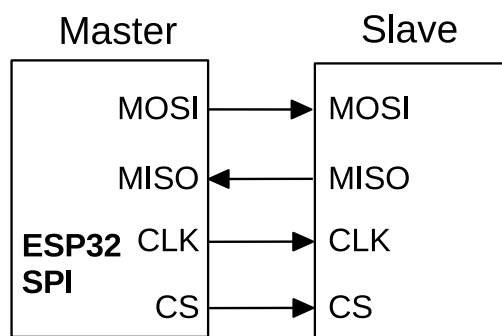
Figure 20.3-1. SPI Master and Slave Full-duplex/Half-duplex Communication
