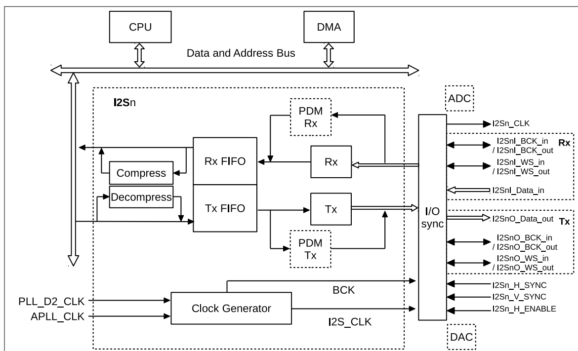
Figure 22.1-1. I2S System Block Diagram
