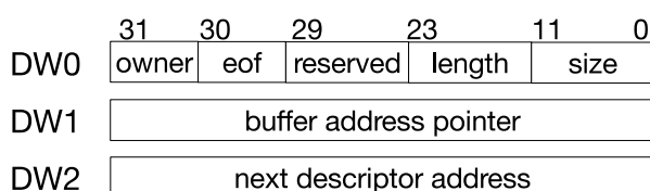
Figure 2.3-2. Linked List Structure
