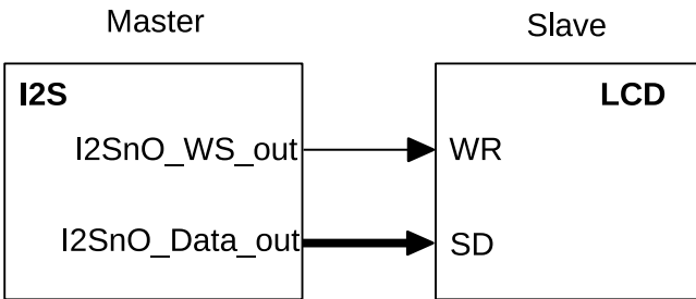
Figure 22.5-1. LCD Master Transmitting Mode
