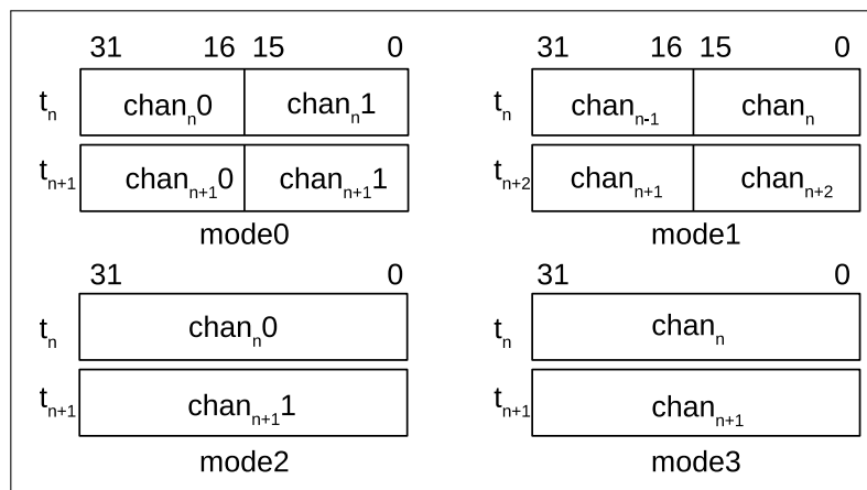
Figure 22.4-6. Modes of Writing Received Data into FIFO
