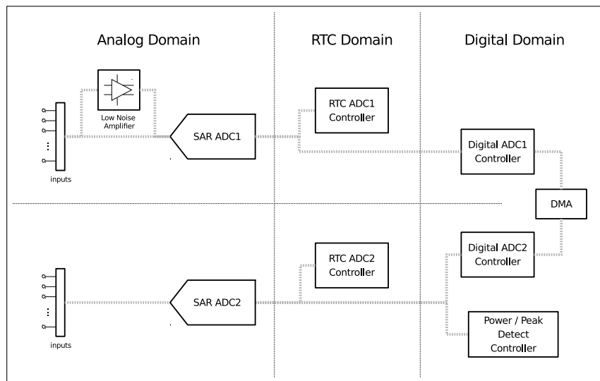
Figure 31.3-1. SAR ADC Depiction
