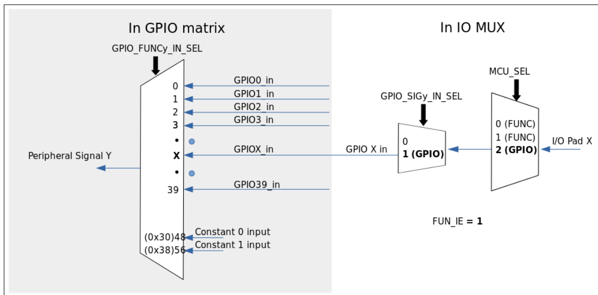
Figure 6.2-1. Peripheral Input via IO MUX, GPIO Matrix
