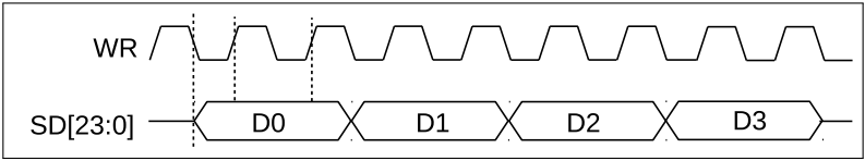
Figure 22.5-2. LCD Master Transmitting Data Frame, Form 1
