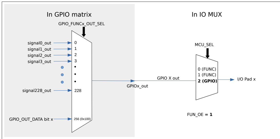
Figure 6.3-1. Output via GPIO Matrix
