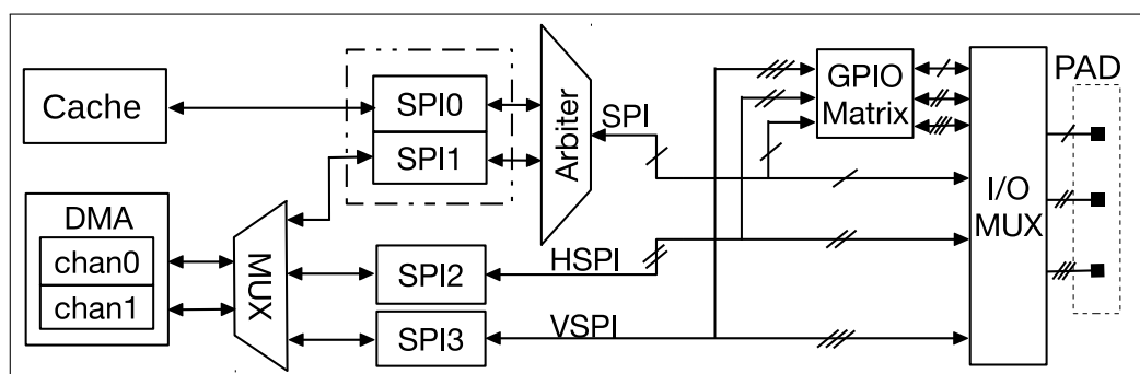
Figure 20.1-1. SPI Architecture
