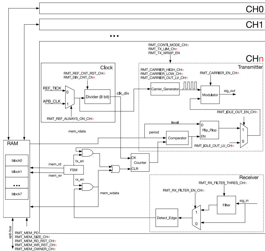
Figure 30.2-1. RMT Architecture
