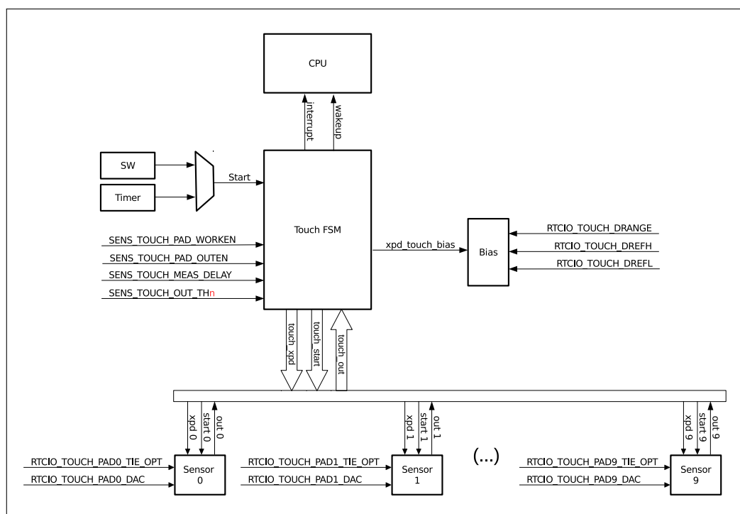
Figure 31.2-4. Touch FSM Structure
