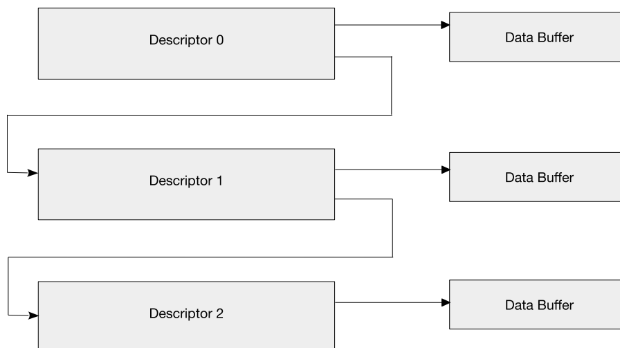
Figure 27.7-1. Descriptor Chain
