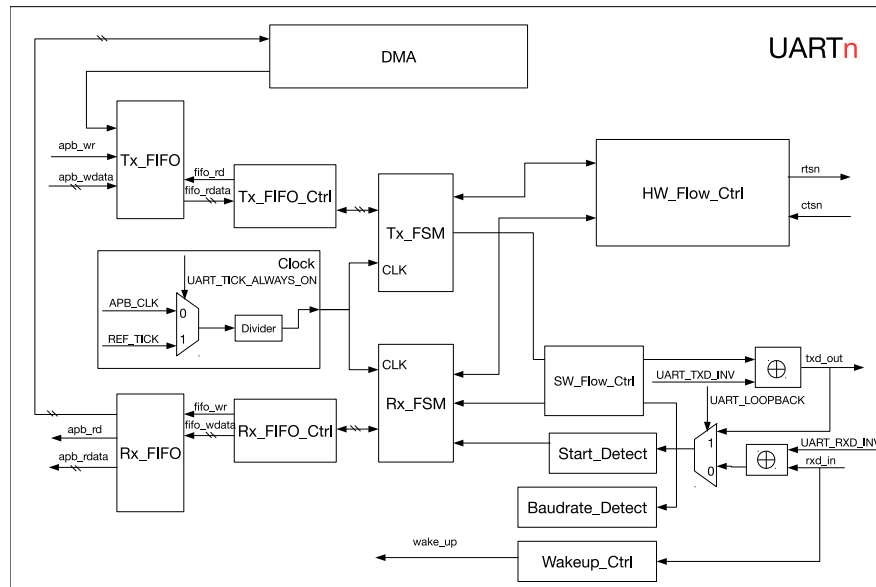
Figure 19.3-1. UART Basic Structure
