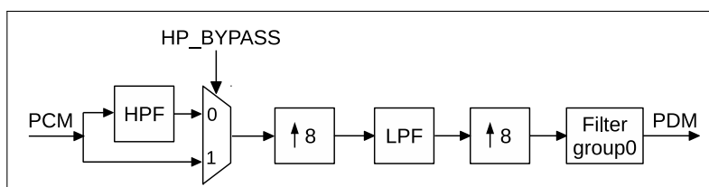
Figure 22.4-7. PDM Transmitting Module
