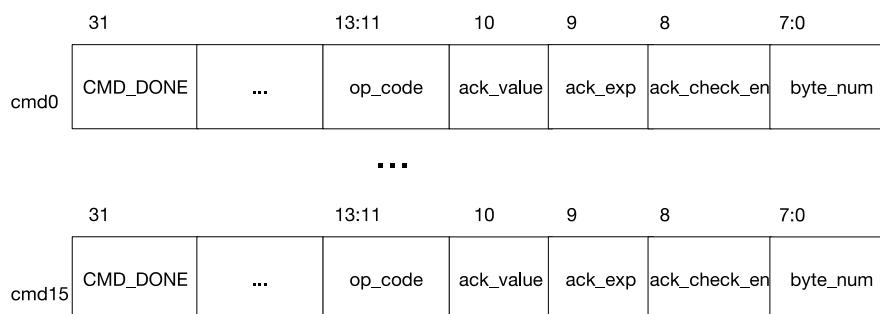
Figure 21.3-4. Structure of The I2C Command Register
