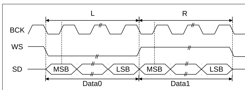
Figure 22.4-2. MSB Alignment Standard
