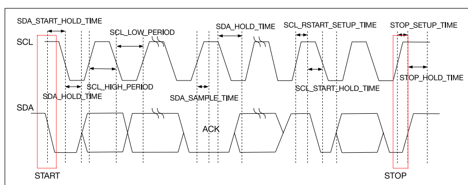
Figure 21.3-3. I2C Sequence Chart
