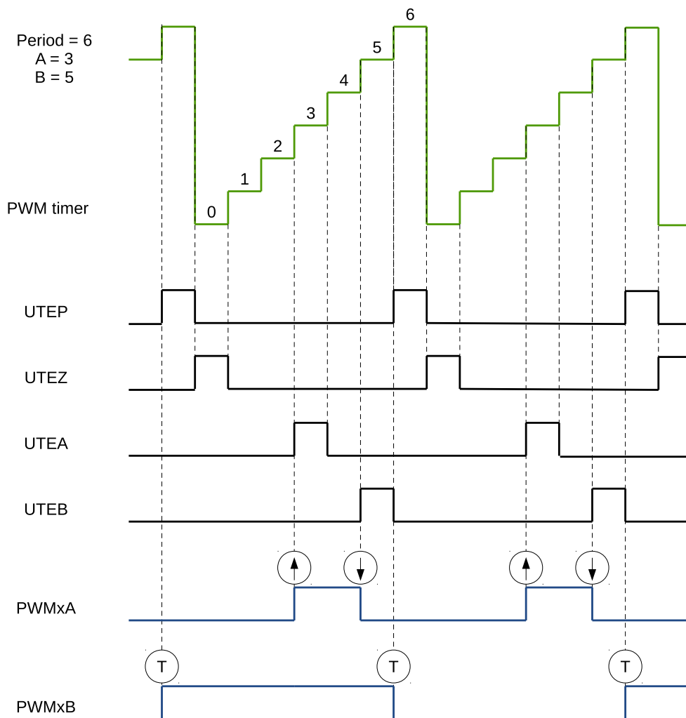
Figure 29.3-16. Count-Up, Pulse Placement Asymmetric Waveform with Independent Modulation on PWMxA
