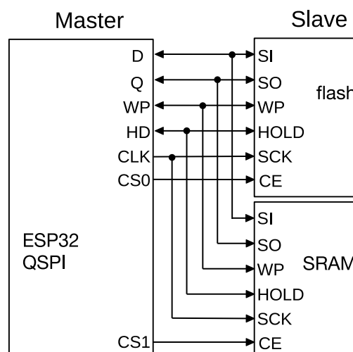
Figure 20.5-1. Parallel QSPI
