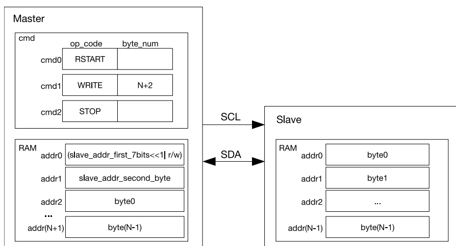
Figure 21.3-6. I2C Master Writes to Slave with 10-bit Address
