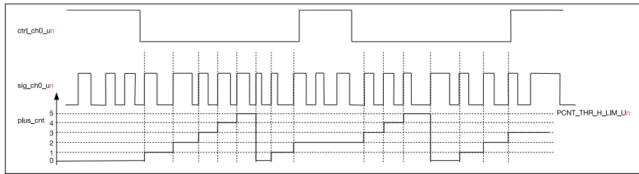
Figure 23.2-2. PULSE_CNT Upcounting Diagram
