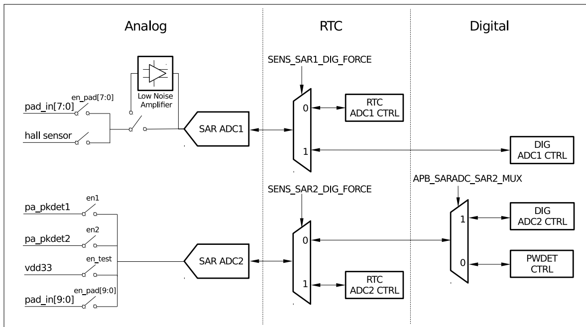
Figure 31.3-2. SAR ADC Outline of Function
