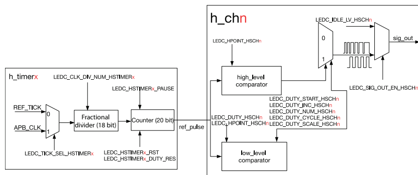
Figure 28.2-2. LED_PWM High-speed Channel Diagram
