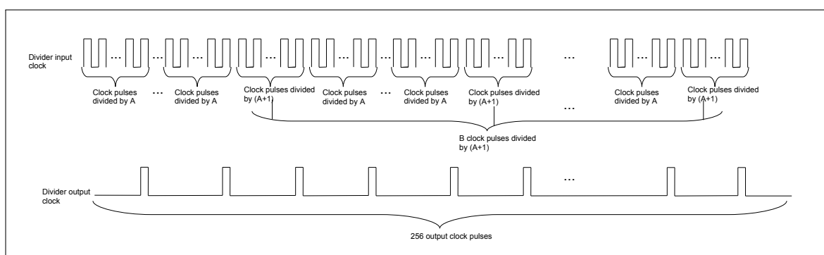
Figure 28.2-3. LED_PWM Divider
