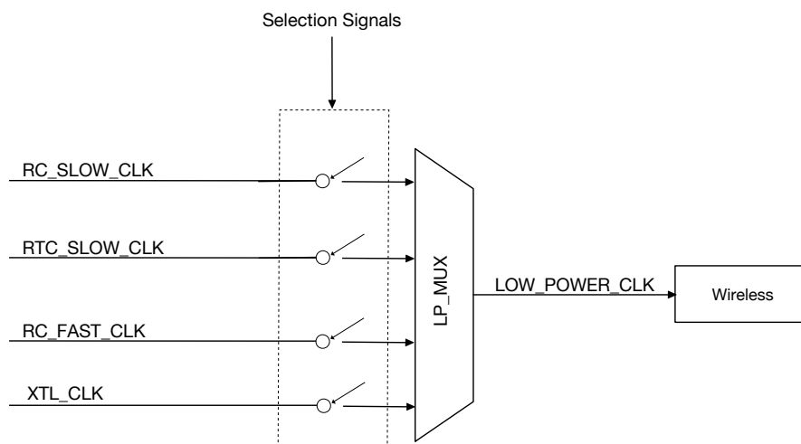
Figure 9.3-7. Digital Low-Power Clocks
