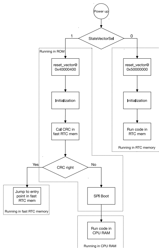
Figure 9.3-10. ESP32 Boot Flow
