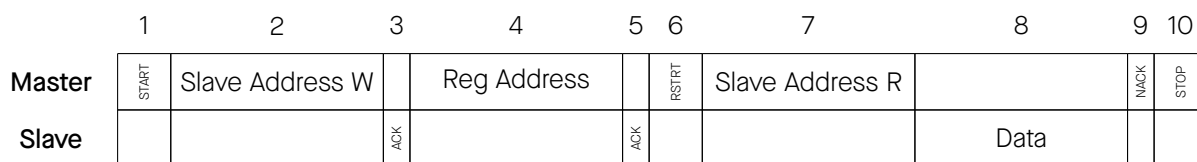
Figure 1.6-1. I2C Read Operation
