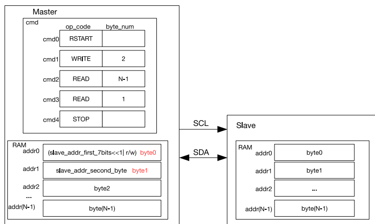
Figure 21.3-10. Master Reads from Slave with 10-bit Address
