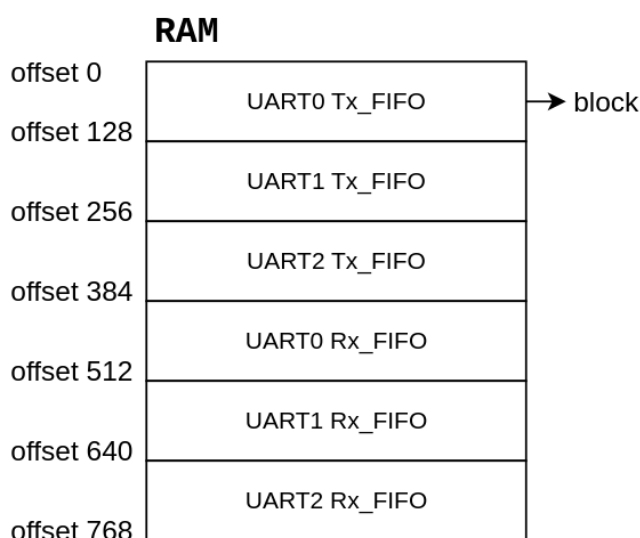
Figure 19.3-2. UART Shared RAM
