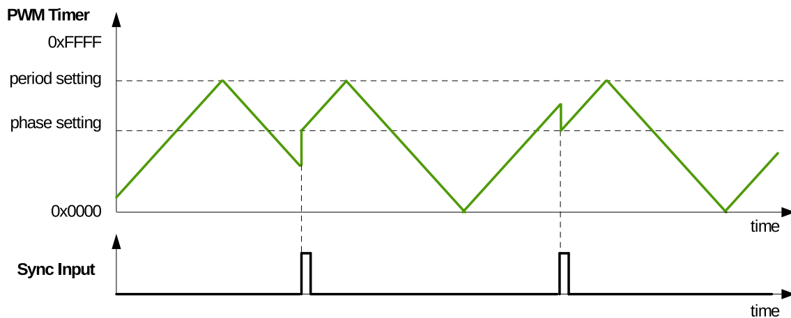
Figure 29.3-9. Count-Up-Down Mode Waveforms, Count-Up at Synchronization Event
