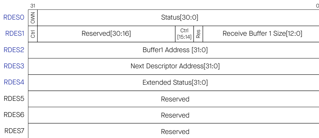
Figure 24.8-2. Receive Descriptor
