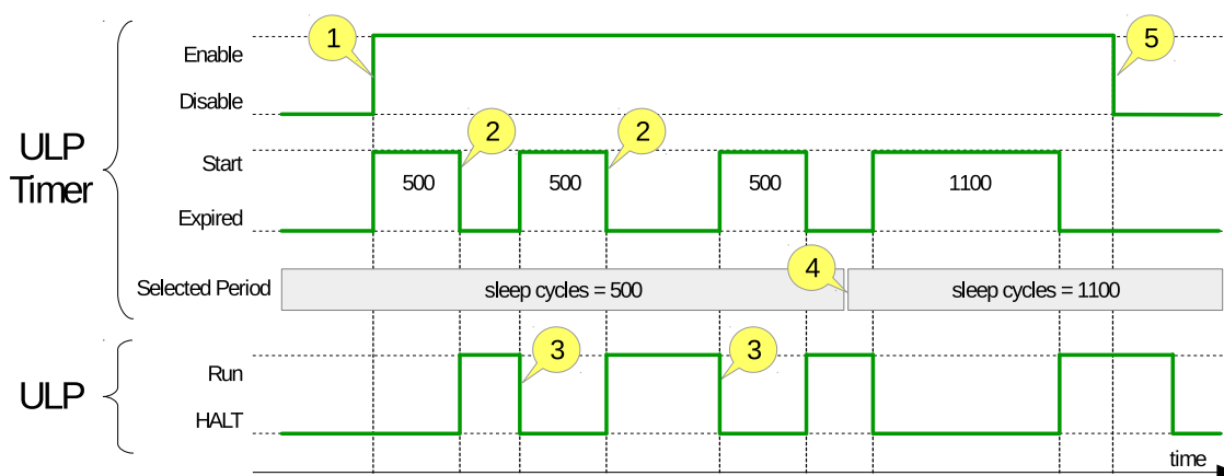
Figure 1.5-2. Sample of a ULP Operation Sequence
