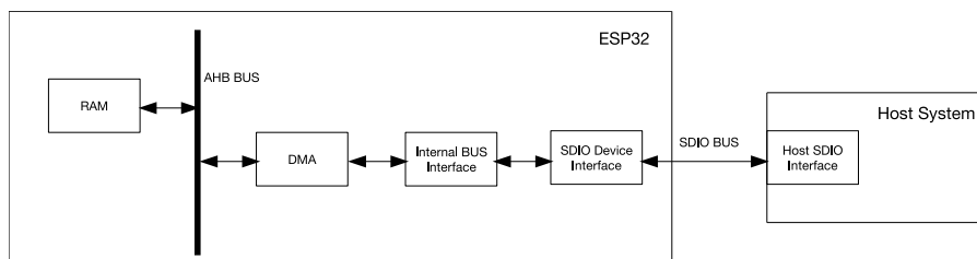
Figure 26.3-1. SDIO Slave Block Diagram
