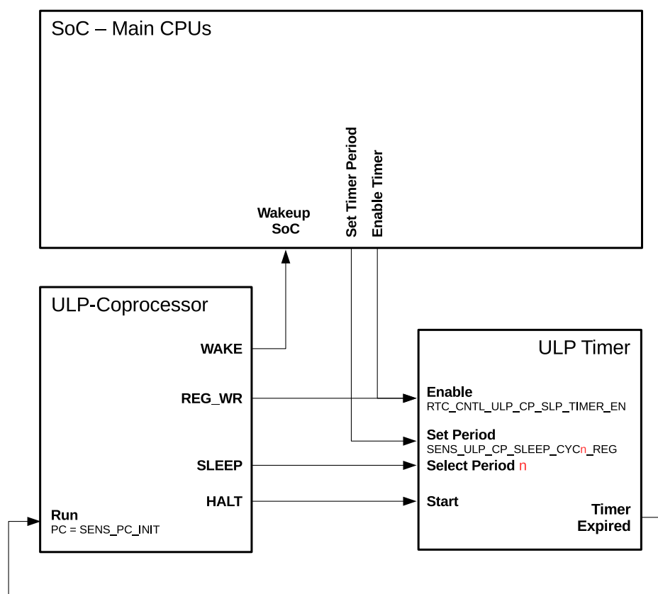
Figure 1.5-1. Control of ULP Program Execution
