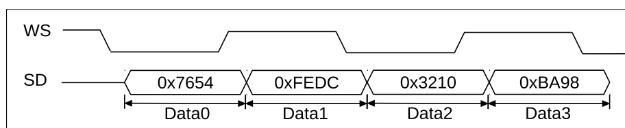
Figure 22.4-5. The First Stage of Receiving Data
