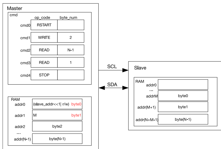
Figure 21.3-11. Master Reads N Bytes of Data from addrM in Slave with 7-bit Address
