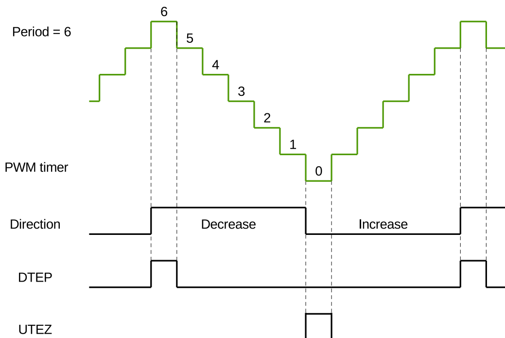
Figure 29.3-12. DTEP and UTEZ Generation in Count-Up-Down Mode
