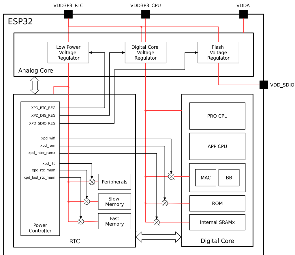
Figure 9.2-1. ESP32 Power Control
