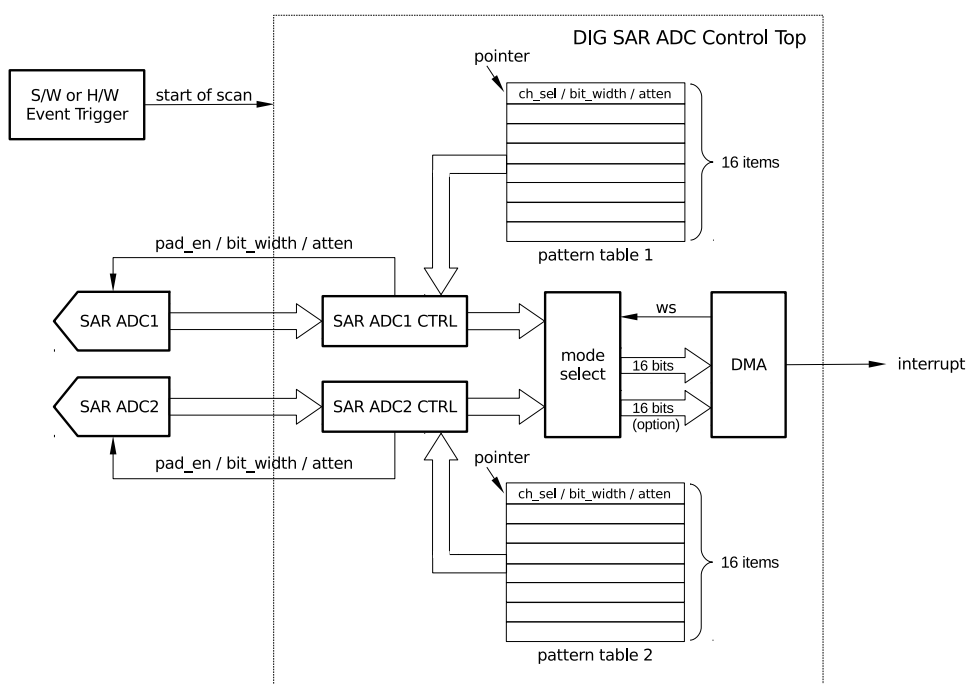
Figure 31.3-4. Diagram of DIG SAR ADC Controllers
