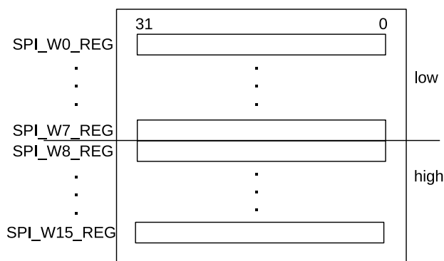
Figure 20.3-2. SPI Data Buffer
