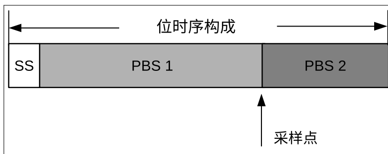
Figure 25.3-5. Layout of a Bit
