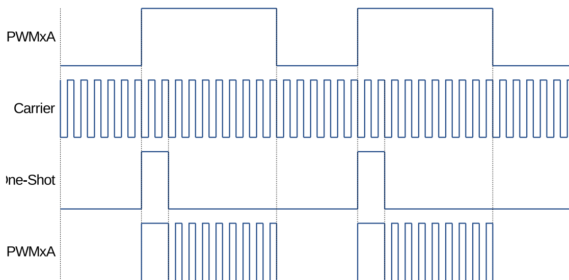
Figure 29.3-27. Example of the First Pulse and the Subsequent Sustaining Pulses of the PWM Carrier Sub-module
