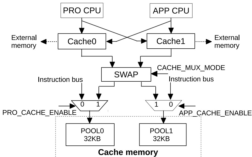
Figure 3.3-1. Cache Block Diagram
