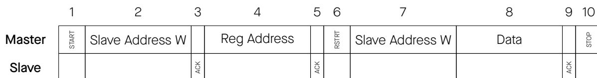
Figure 1.6-2. I2C Write Operation
