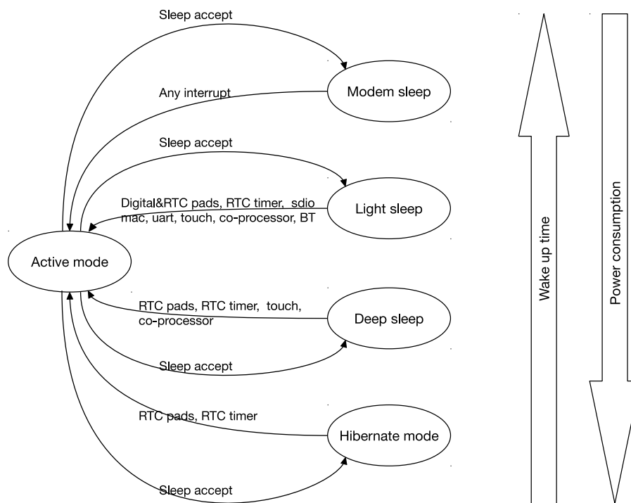
Figure 9.3-9. Power Modes
