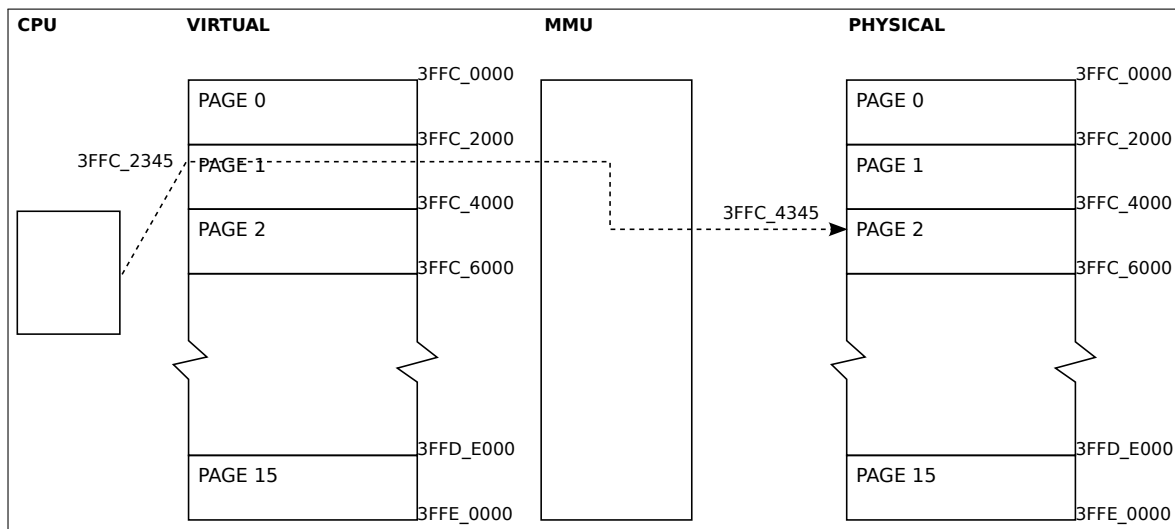
Figure 4.3-1. MMU Access Example
