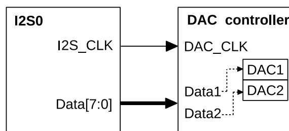
Figure 22.5-6. DAC Interface of I2S
