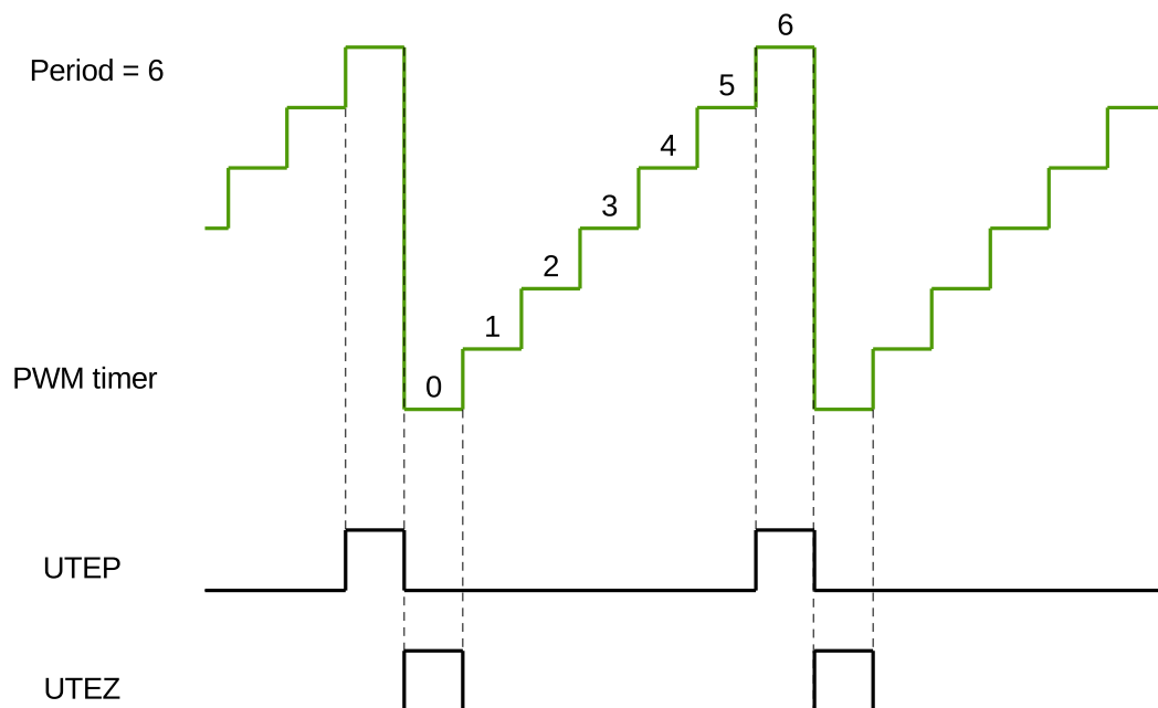
Figure 29.3-10. UTEP and UTEZ Generation in Count-Up Mode
