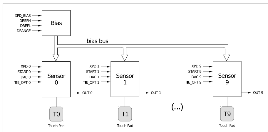
Figure 31.2-2. Touch Sensor Structure
