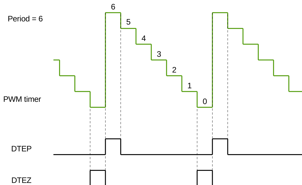
Figure 29.3-11. DTEP and DTEZ Generation in Count-Down Mode
