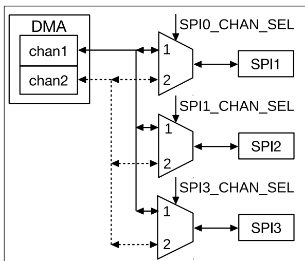
Figure 2.5-1. SPI DMA
