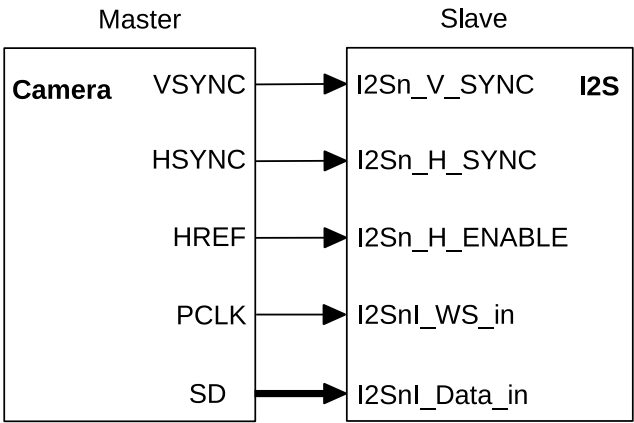
Figure 22.5-4. Camera Slave Receiving Mode
