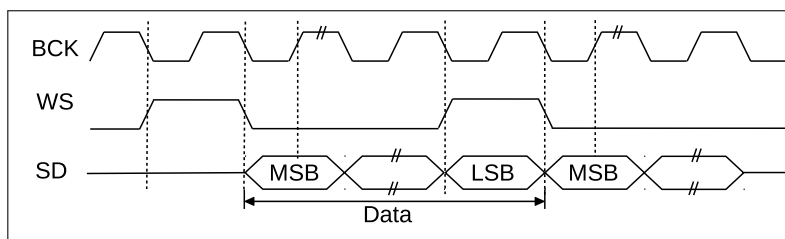
Figure 22.4-3. PCM Standard
