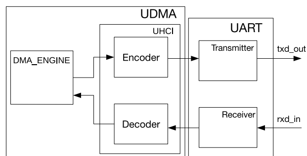
Figure 2.4-1. Data Transfer in UDMA Mode
