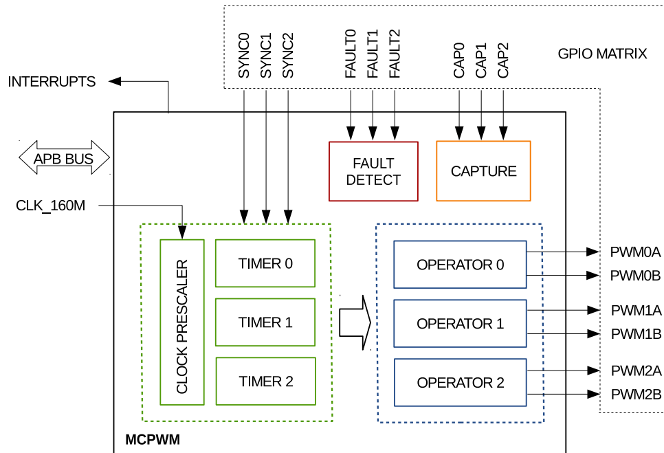
Figure 29.2-1. MCPWM Module Overview
