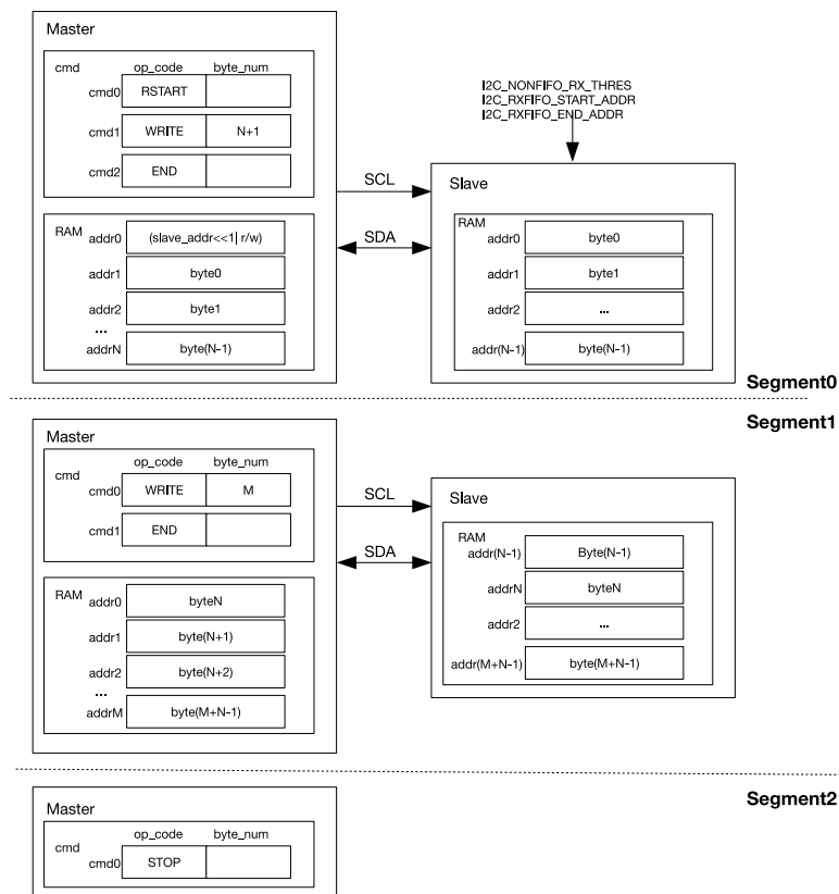
Figure 21.3-8. Master Writes to Slave with 7-bit Address in Three Segments
