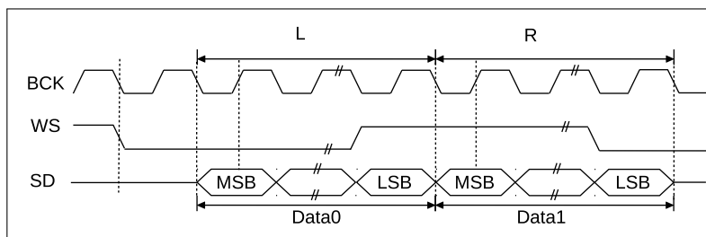
Figure 22.4-1. Philips Standard
