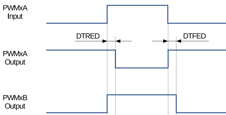
Figure 29.3-23. Active Low Complementary (ALC) Dead Time Waveforms
