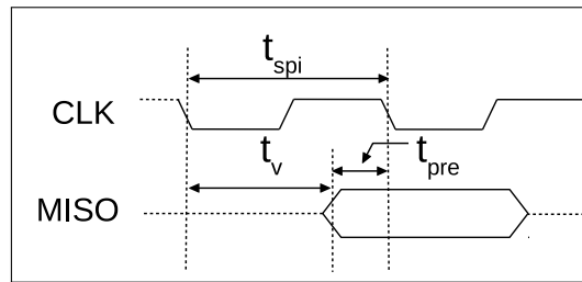
Figure 20.4-1. GP-SPI Slave Data Output
