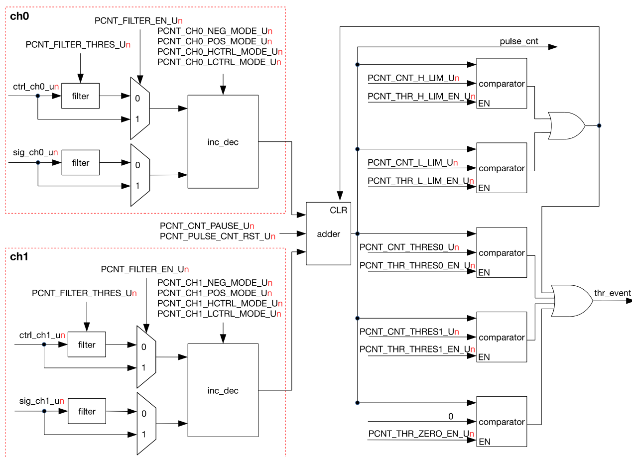
Figure 23.2-1. PULSE_CNT Architecture
