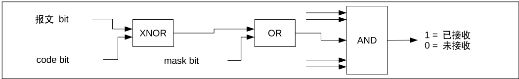
Figure 25.5-1. Acceptance Filter
