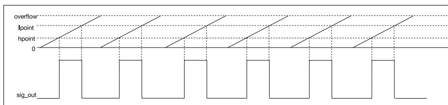
Figure 28.2-4. LED PWM Output Signal Diagram
