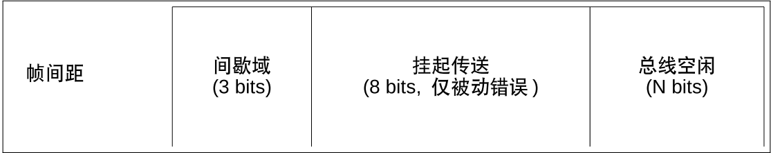
Figure 25.3-4. The Fields within an Interframe Space
