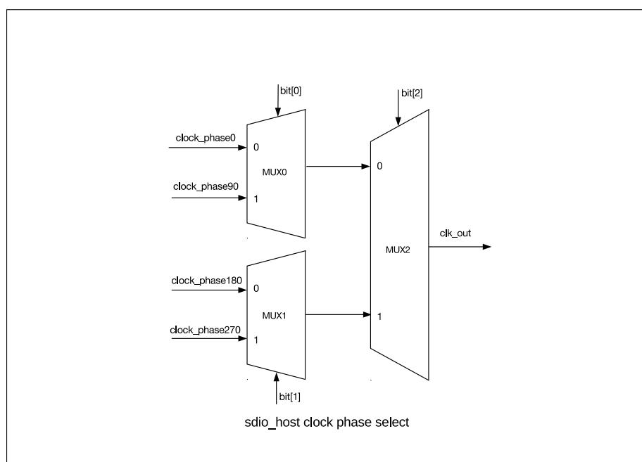
Figure 27.11-1. Clock Phase Selection
