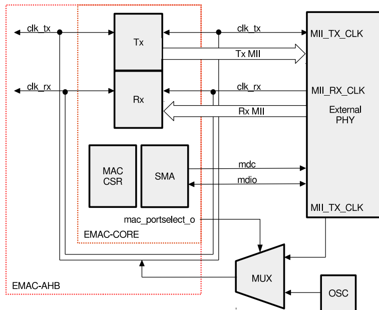
Figure 24.6-2. MII Clock
