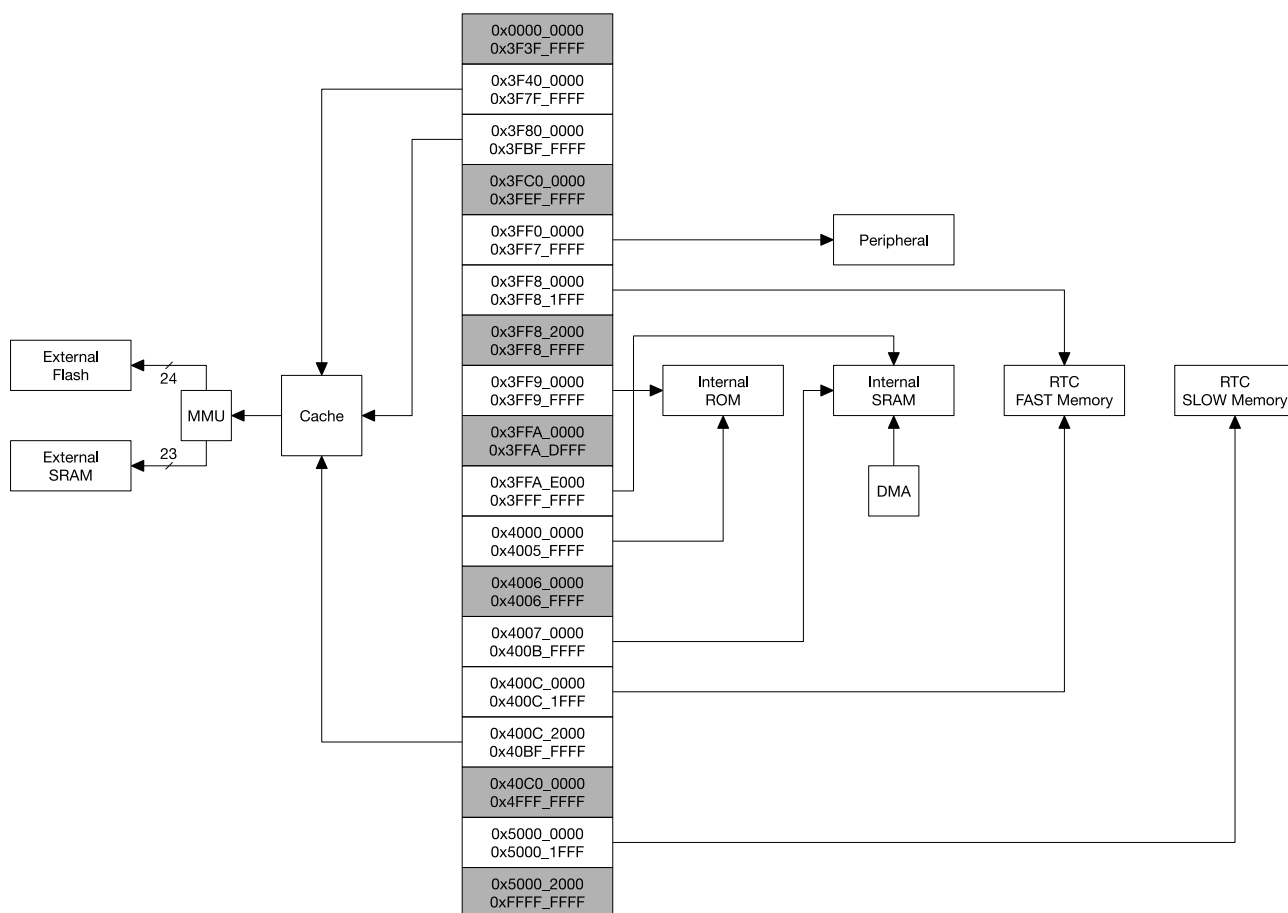
Figure 3.2-2. System Address Mapping
