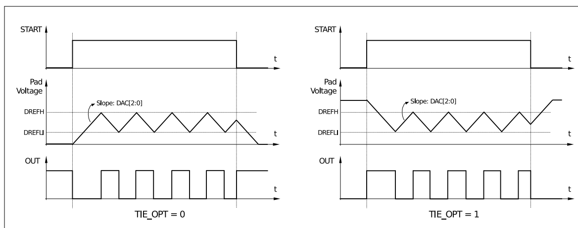
Figure 31.2-3. Touch Sensor Operating Flow
