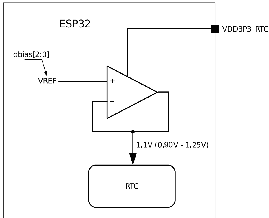
Figure 9.3-2. Low-Power Voltage Regulator
